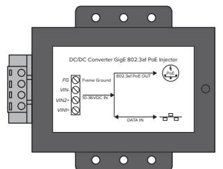
FLIR PoE injector (2nd Generation; 5Gbit) Part: A80811
